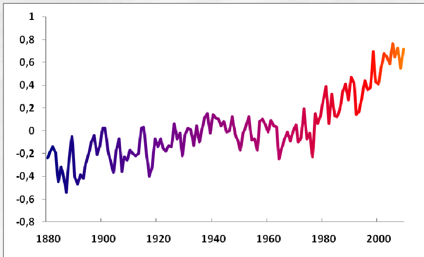
Global Land-Ocean temperature index – 12 months running Mean – NASA – 6 juin 2010
